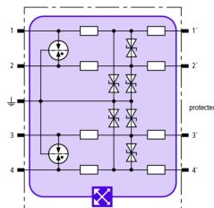
Basic circuit diagram BXT ML4 BE C 24
