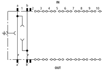
Basic circuit diagram BM 10 DRL
