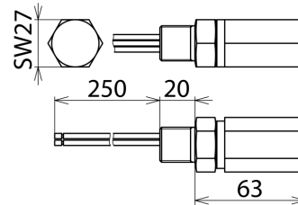
Dimension drawing DPI CD EXI+D 2X48 N
