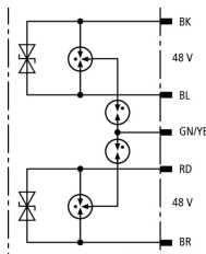
Basic circuit diagram DPI CD EXI+D 2X48 N
