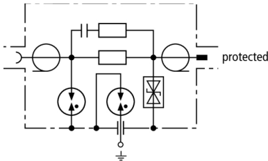
Basic circuit diagram UGKF BNC
