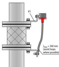
Installation of EXFS L300
