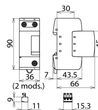
Dimension drawing DGPH M 255
